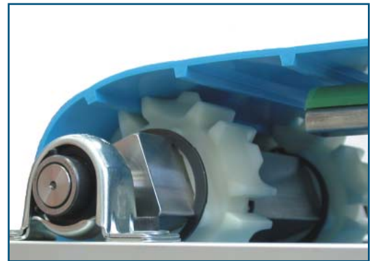
DualDrive with Intralox Series 800 pulleys
